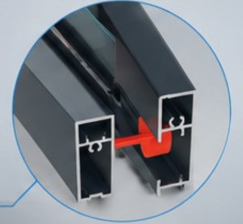
ALT RAY PROFİL BOTTOM RAIL PROFILE
