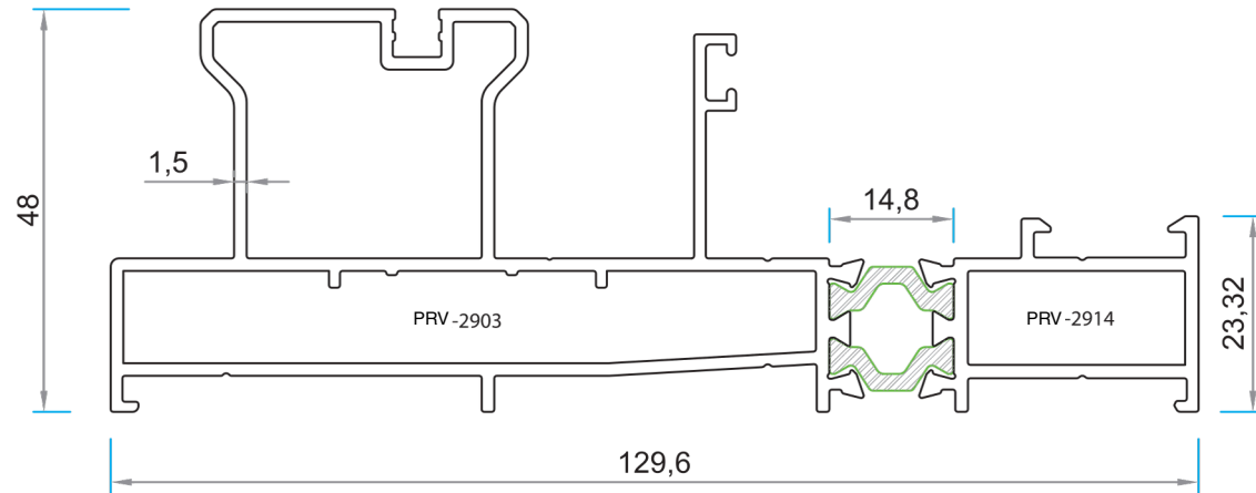
PRV-2944 Ağırlık (kg/mt): 2,133 STATİK / STATIC Jx (cm 4 ): 12,92 Jy (cm 4 ): 109,74
